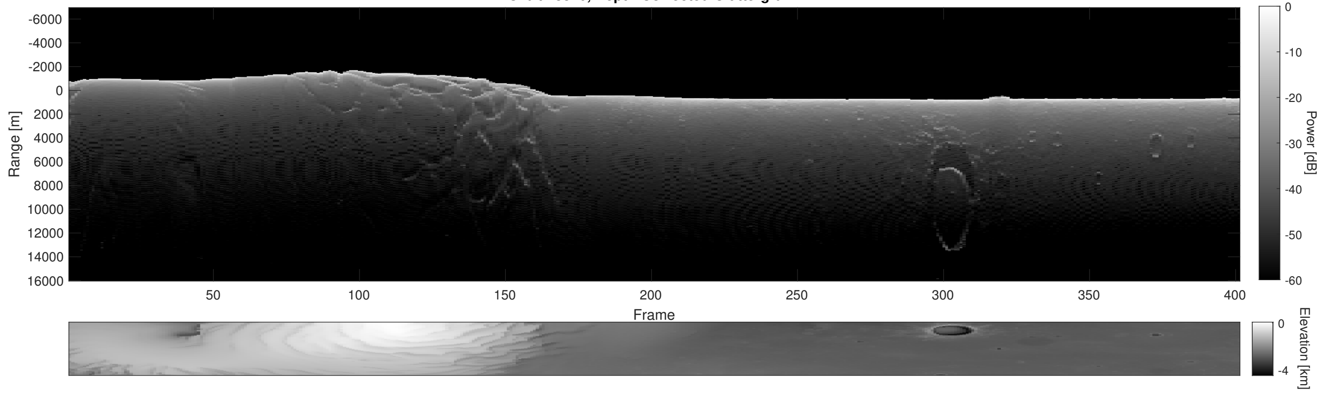
Orbit 18310, Depth-Corrected Cluttergram
