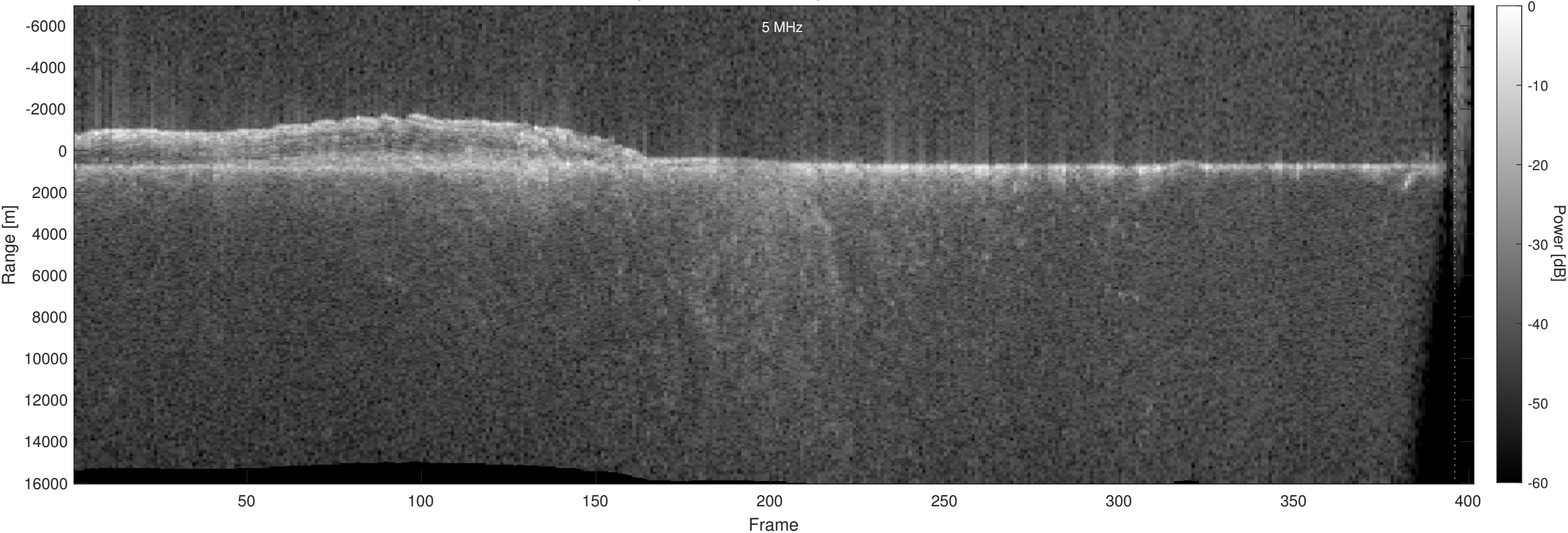
Orbit 18310, Optimized, Window, Depth-Corrected, Channel 2
