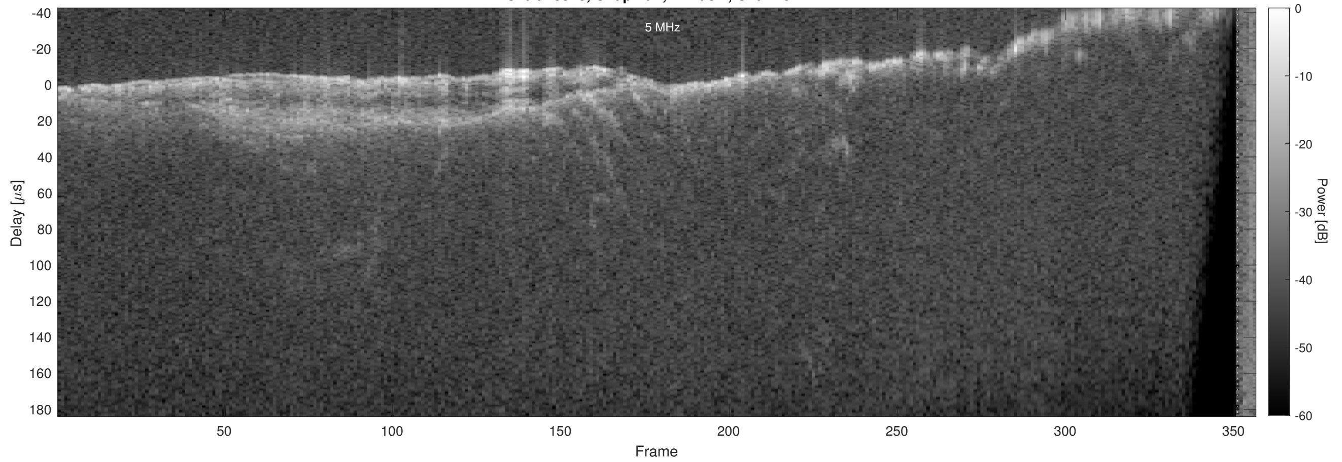
Orbit 18318, Chapman, Window, Channel 2
