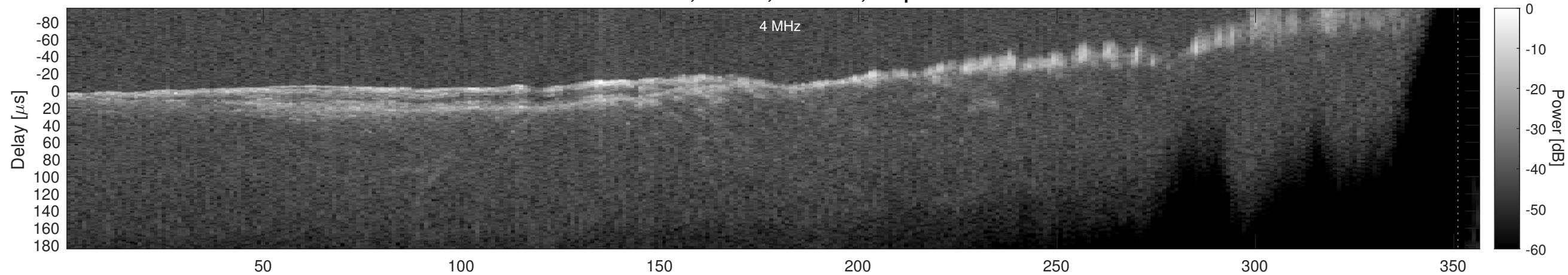
Orbit 18318, Window, Channel 2, Optimized
