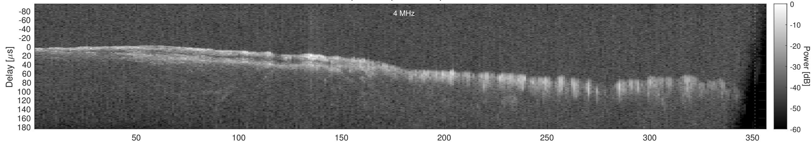
Orbit 18318, Window, Channel 2, Chapman
