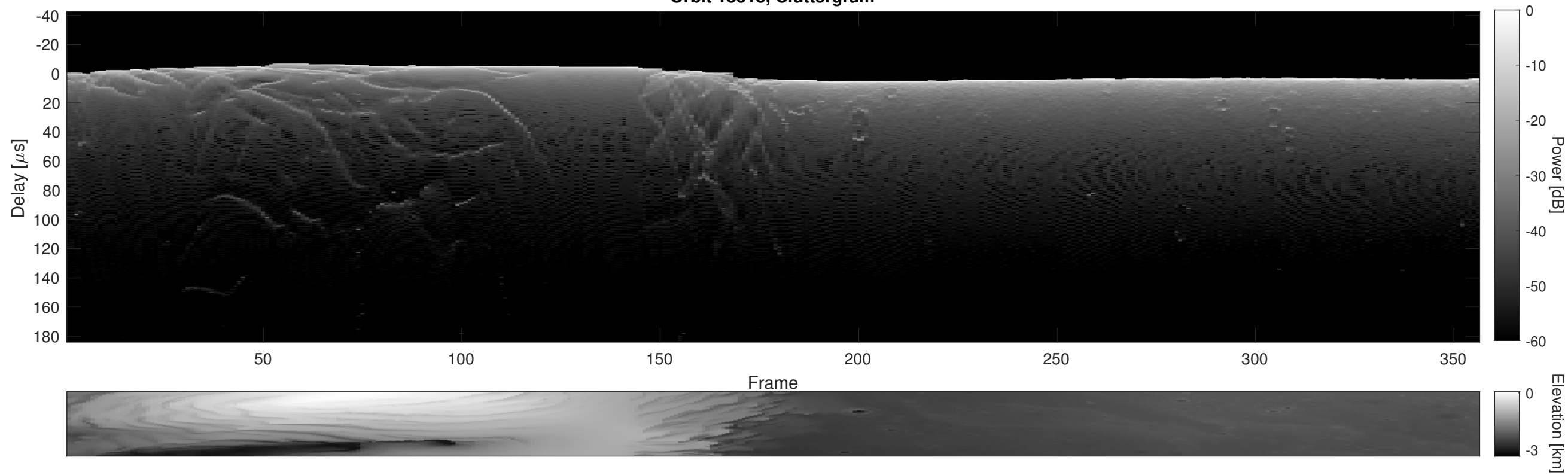
Orbit 18318, Cluttergram
