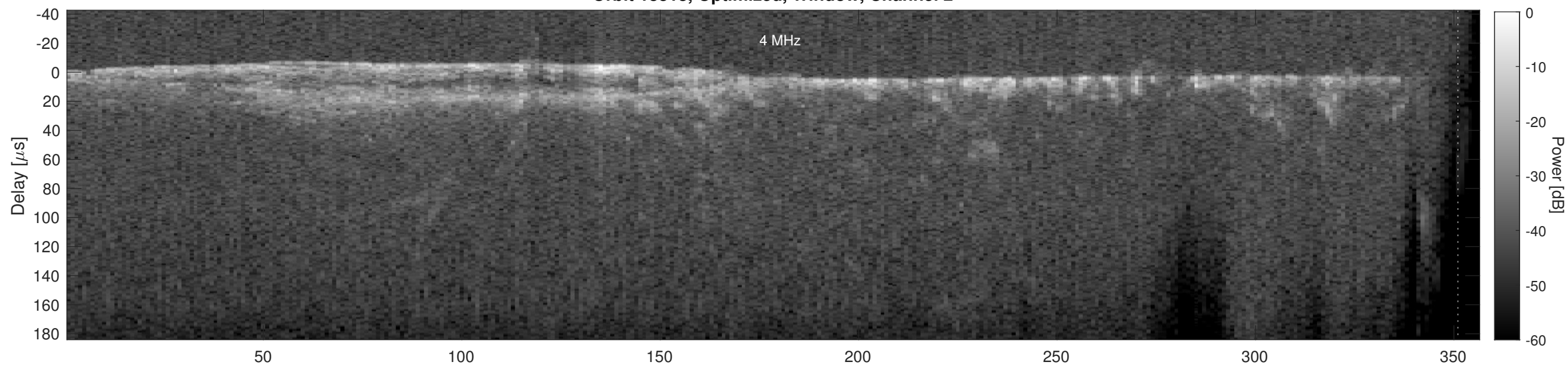
Orbit 18318, Cluttergram
