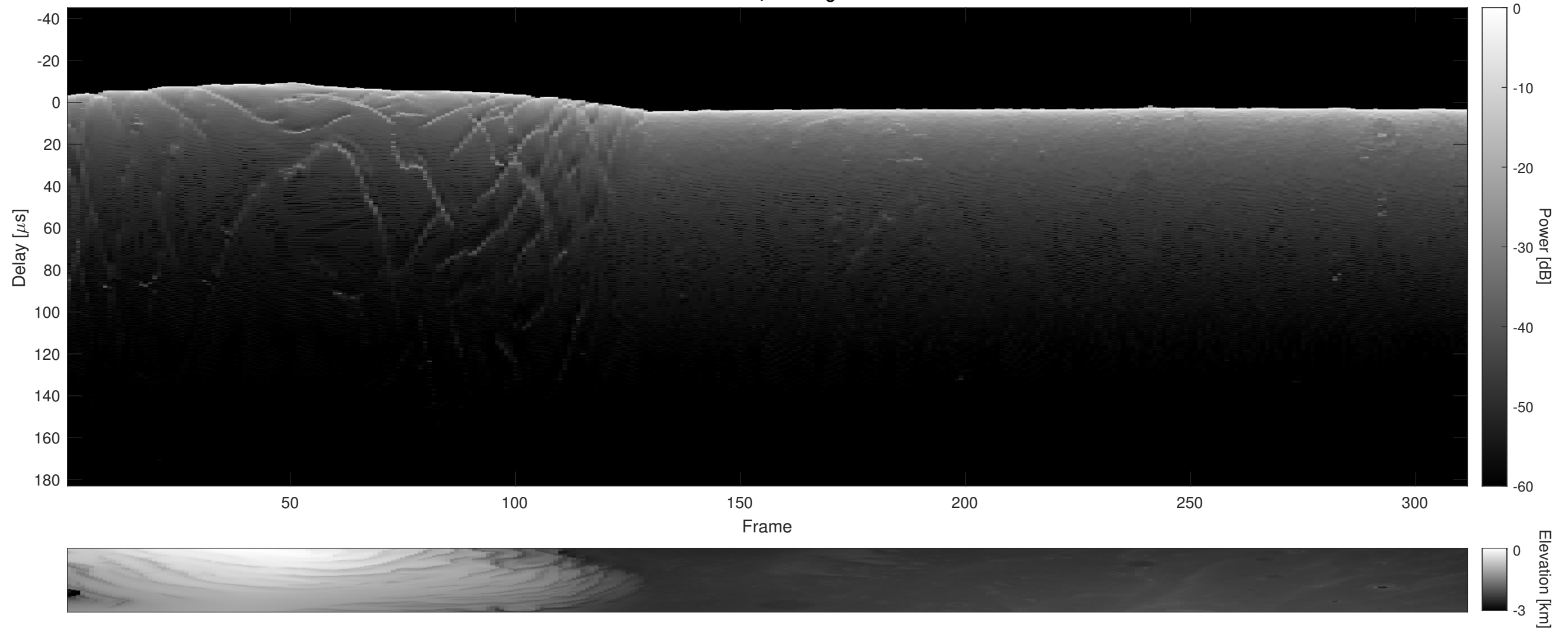
Orbit 18321, Cluttergram
