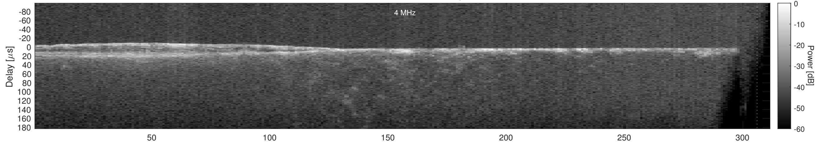
Orbit 18321, Cluttergram
