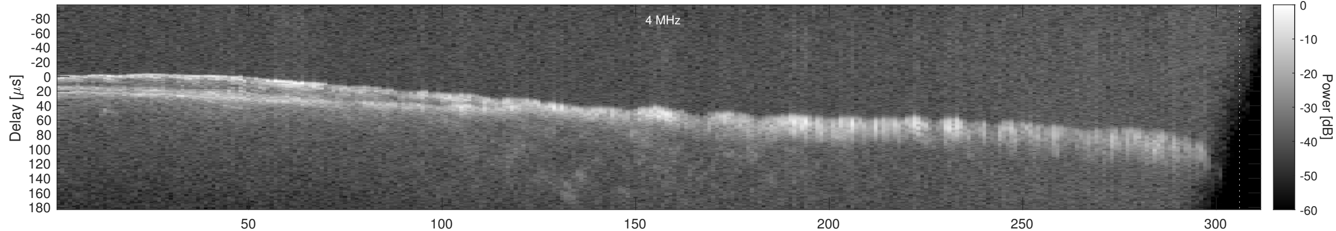
Orbit 18321, Window, Channel 2, Chapman
