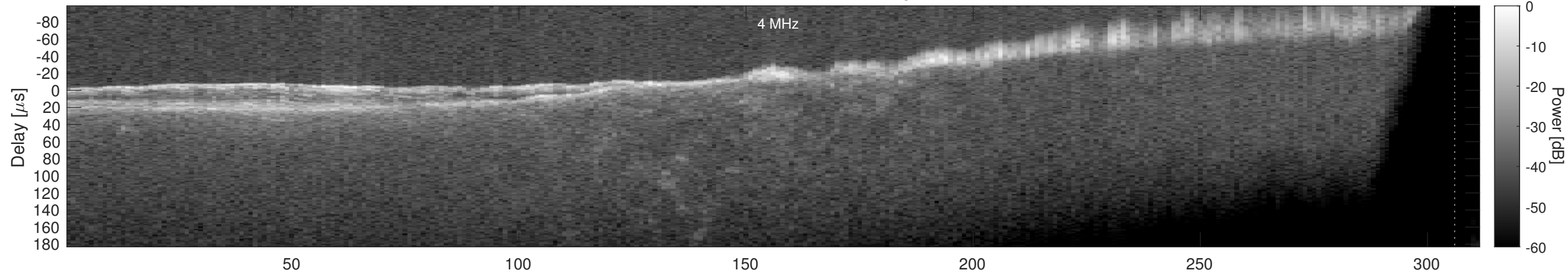
Orbit 18321, Window, Channel 2, Optimized
