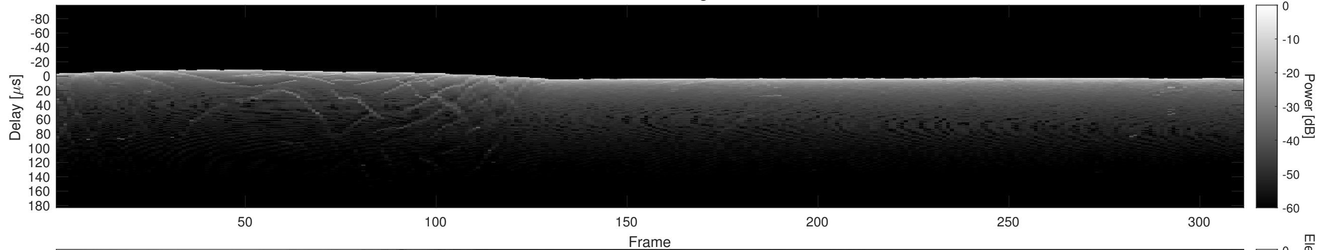
Orbit 18321, Cluttergram
