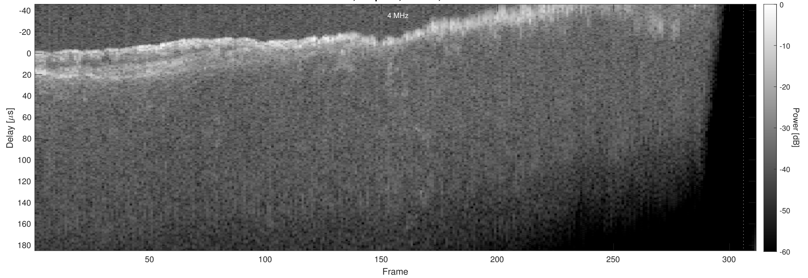
Orbit 18323, Chapman, Window, Channel 2
