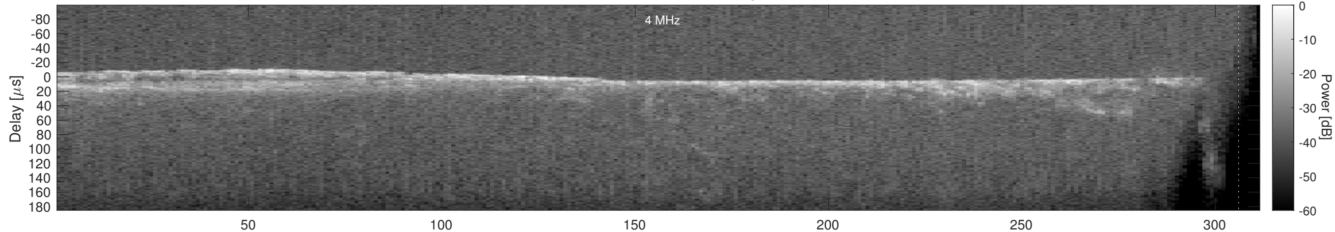
Orbit 18323, Cluttergram
