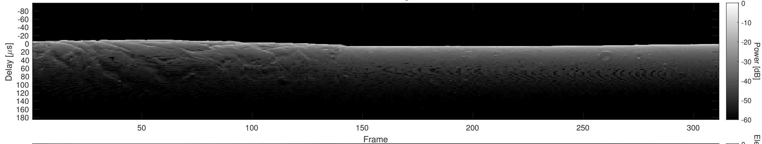
Orbit 18323, Cluttergram
