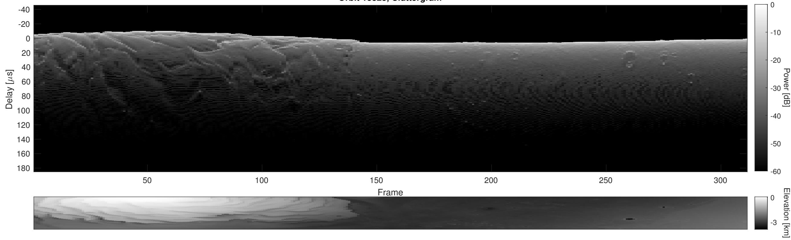
Orbit 18323, Cluttergram
