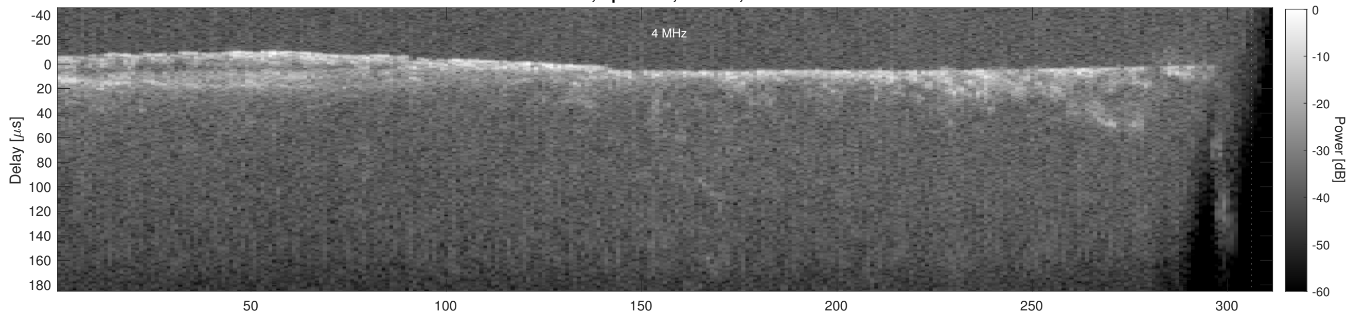
Orbit 18323, Cluttergram
