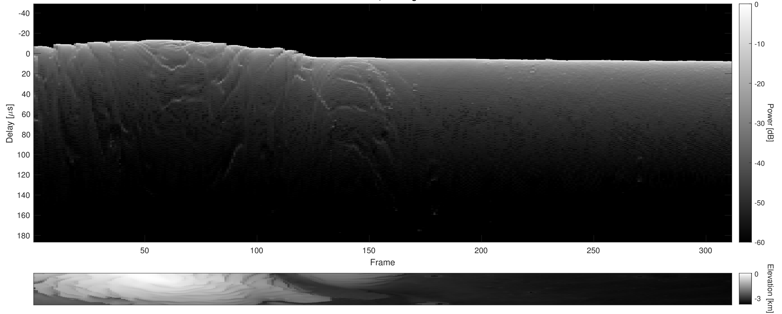
Orbit 18326, Cluttergram
