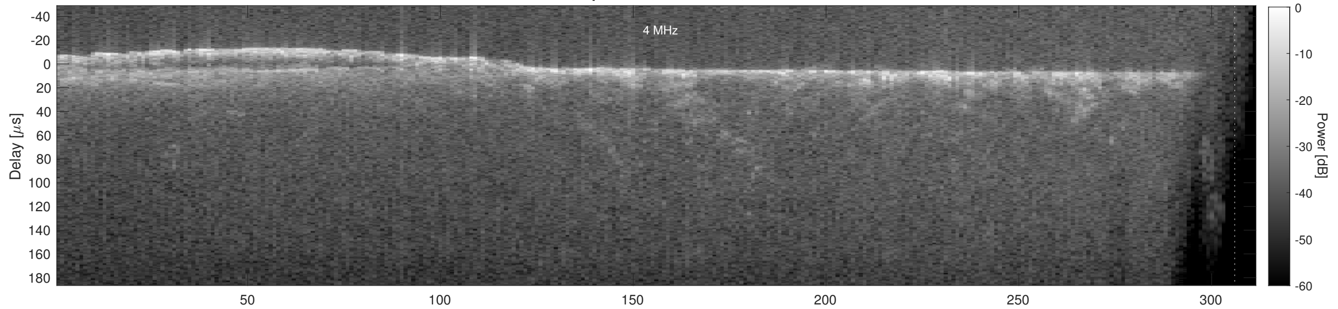
Orbit 18326, Cluttergram
