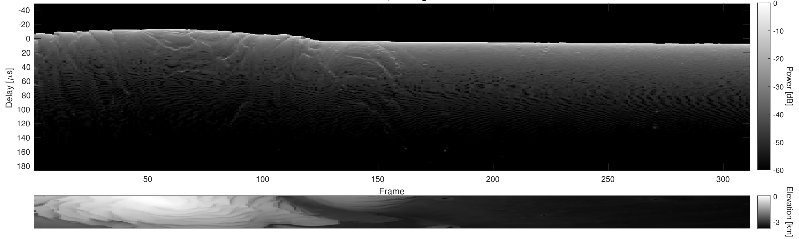
Orbit 18326, Cluttergram
