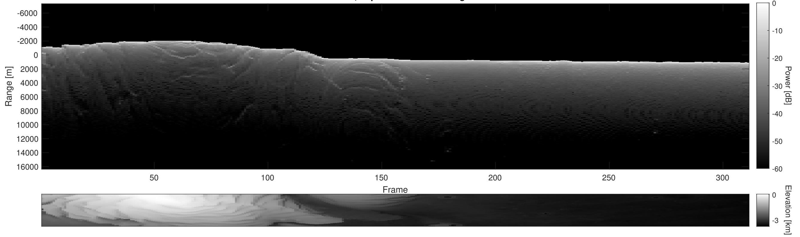
Orbit 18326, Depth-Corrected Cluttergram
