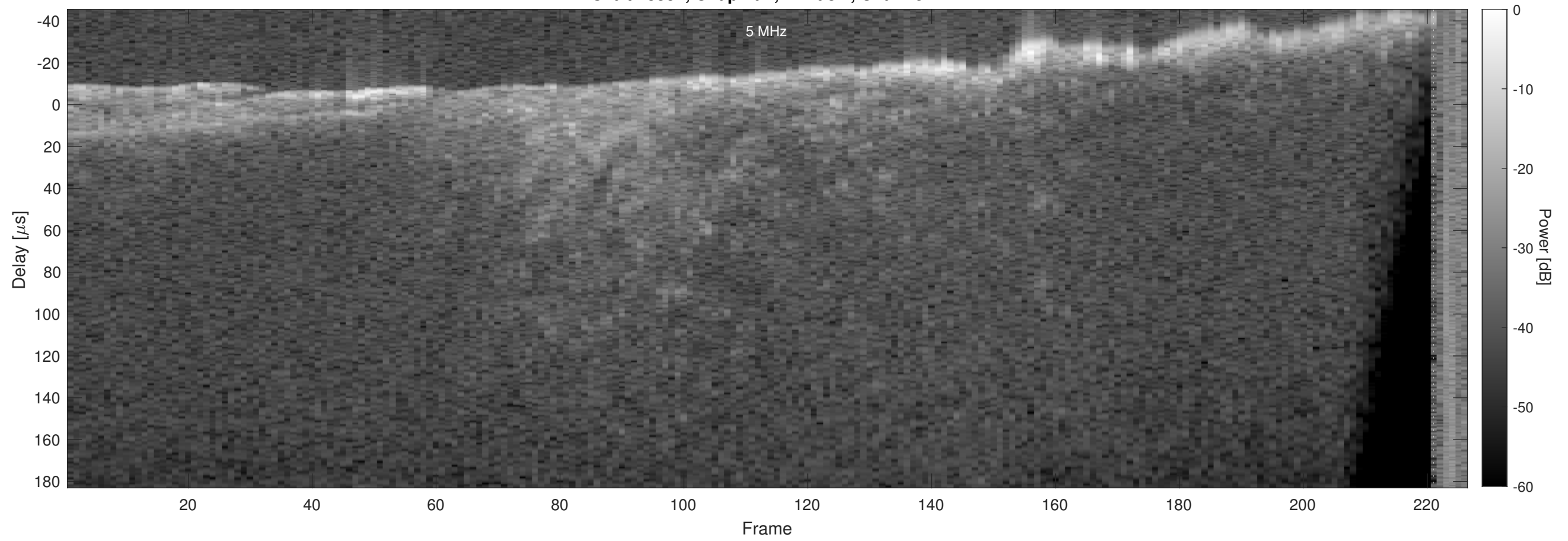
Orbit 18334, Chapman, Window, Channel 2
