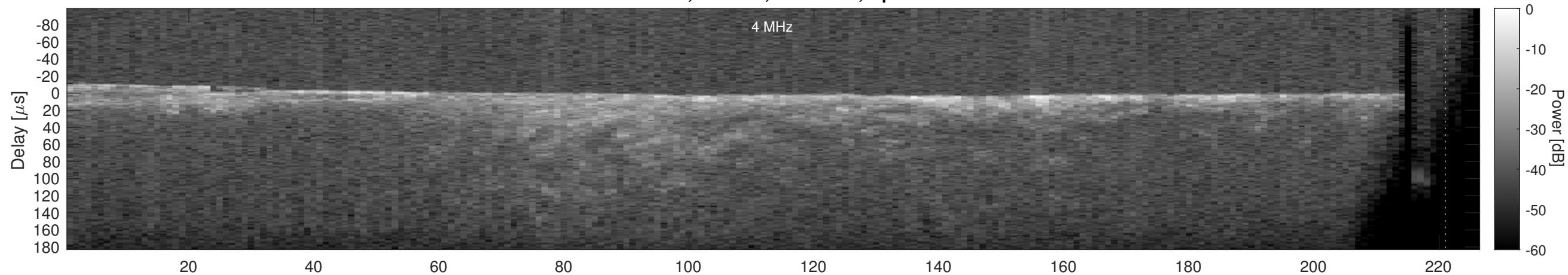
Orbit 18334, Cluttergram
