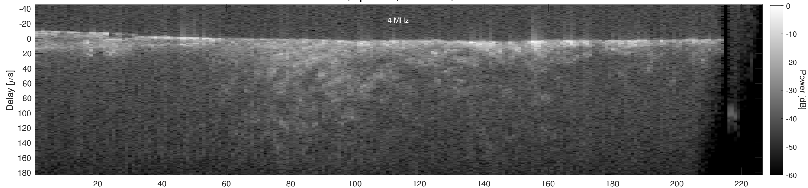
Orbit 18334, Cluttergram
