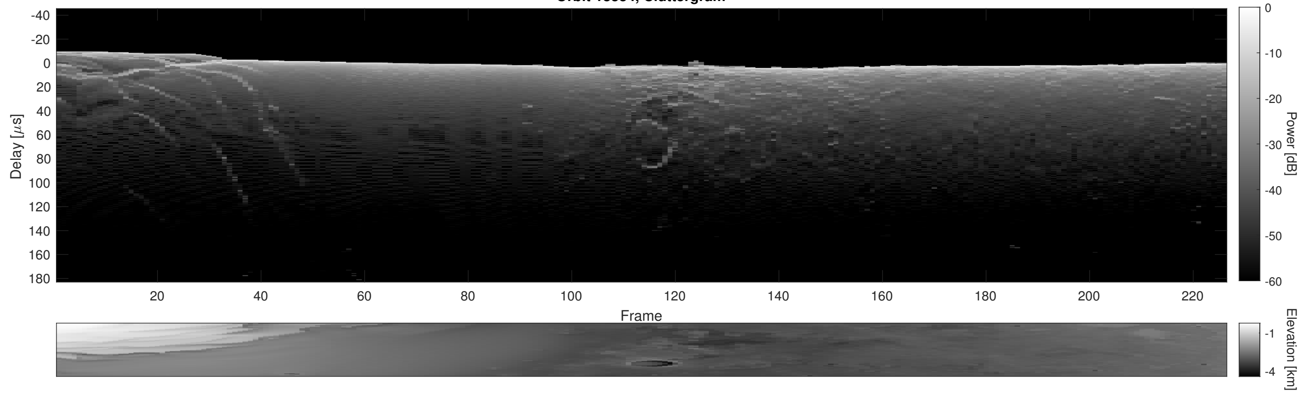
Orbit 18334, Cluttergram
