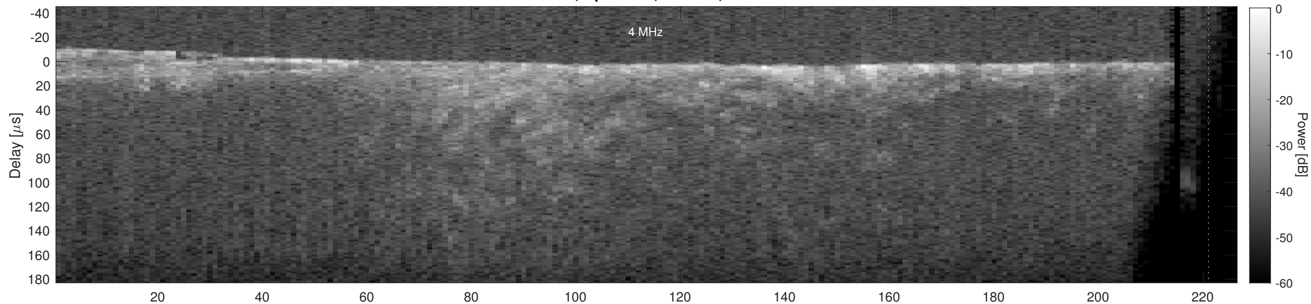
Orbit 18334, Cluttergram
