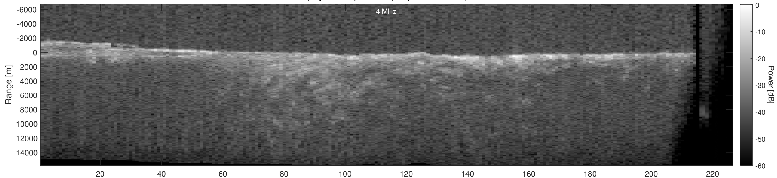
Orbit 18334, Depth-Corrected Cluttergram
