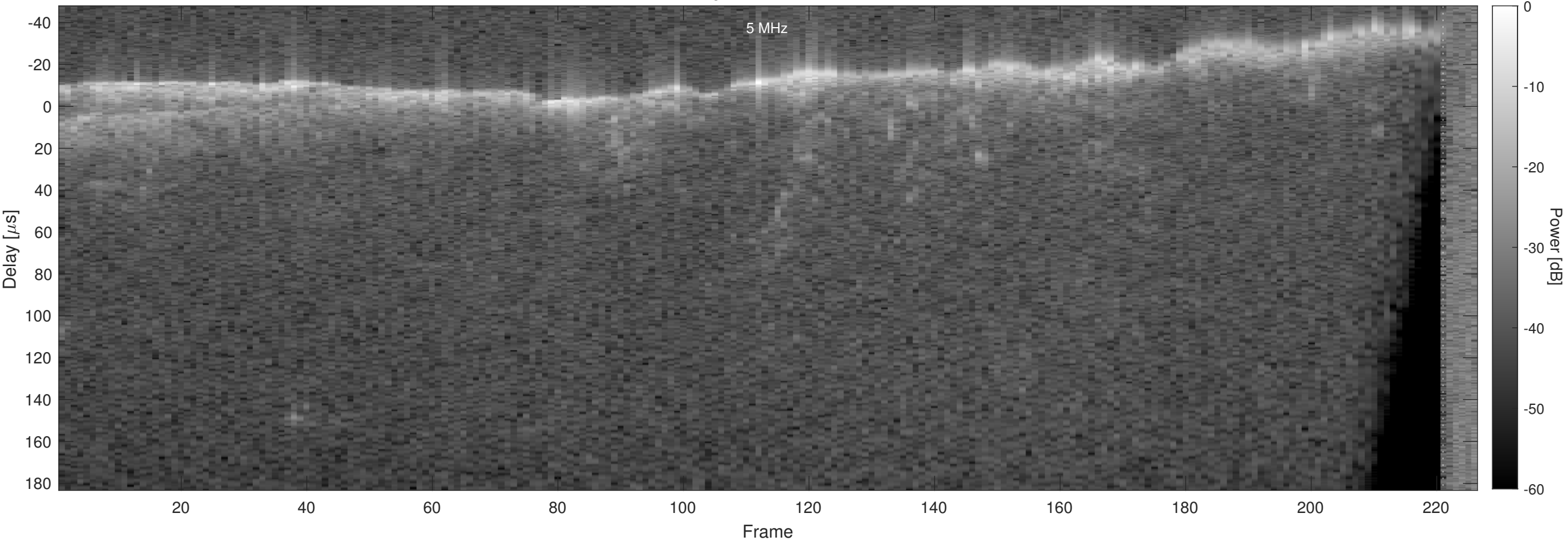
Orbit 18337, Chapman, No Window, Channel 2
