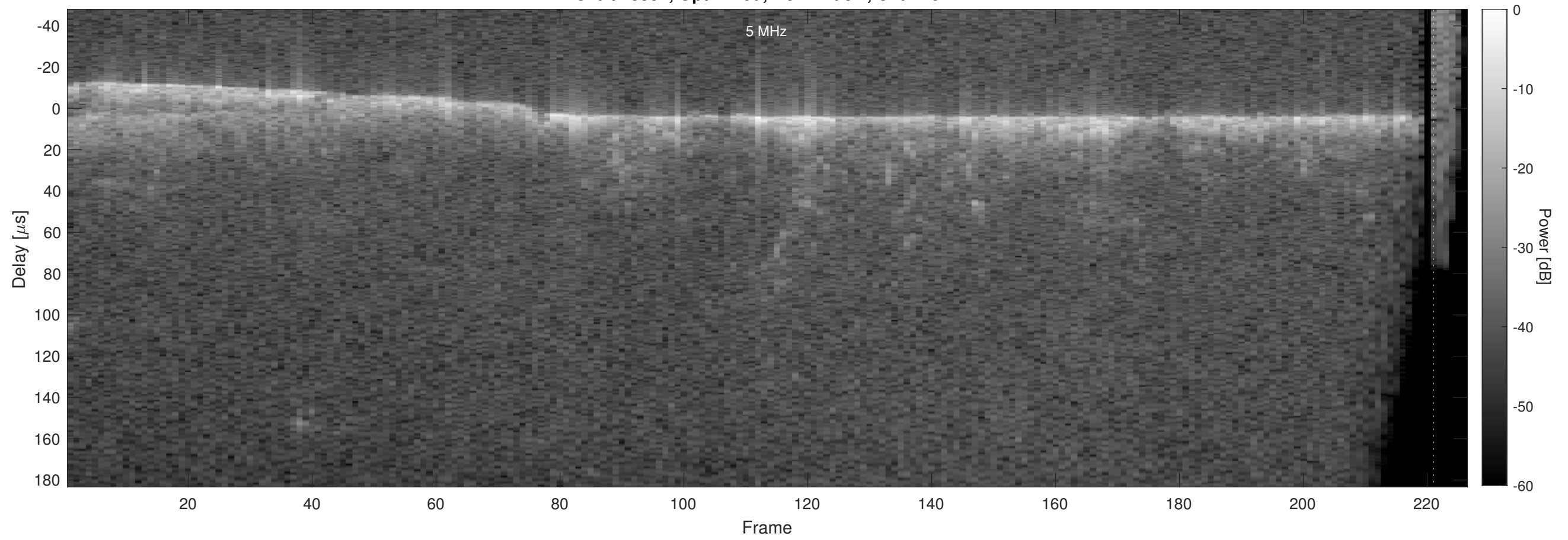
Orbit 18337, Optimized, No Window, Channel 2
