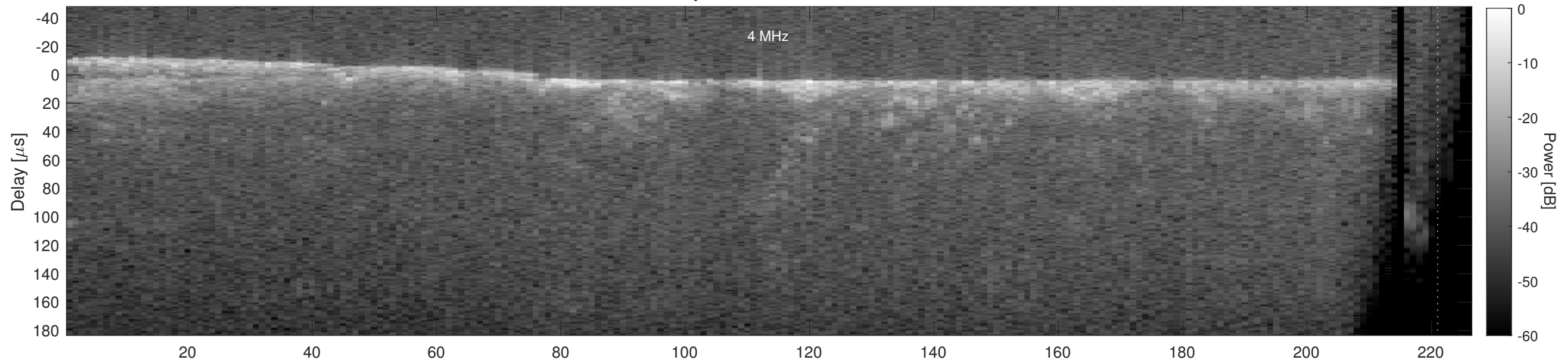
Orbit 18337, Cluttergram
