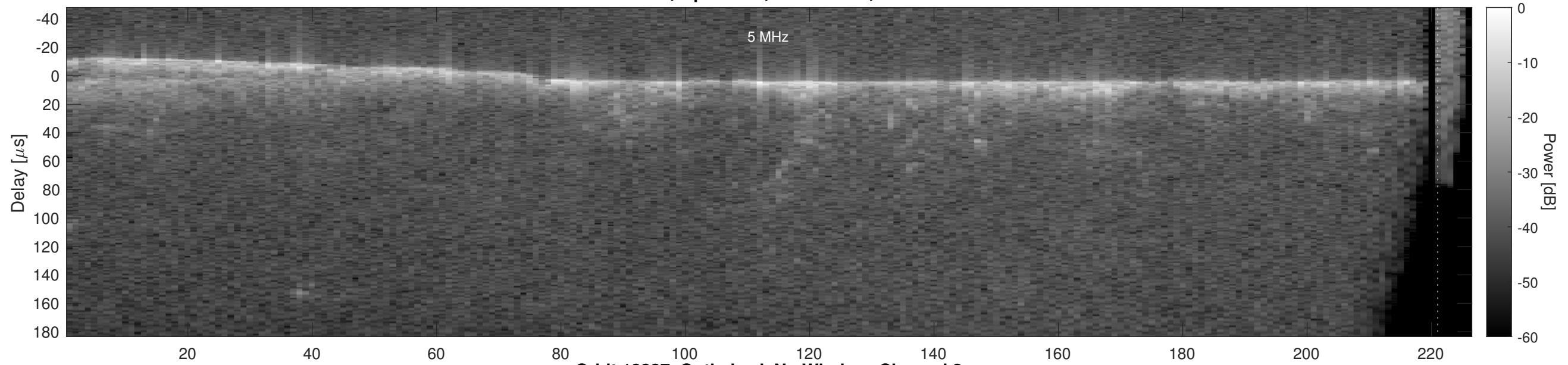
Orbit 18337, Optimized, No Window, Channel 2
