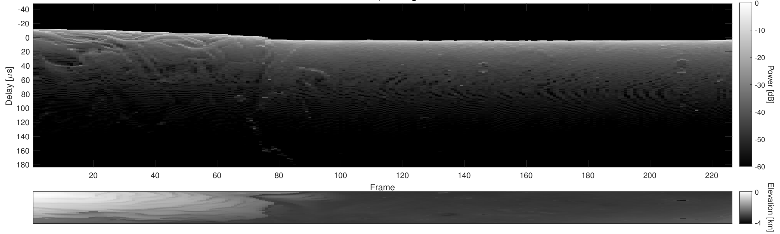
Orbit 18337, Cluttergram
