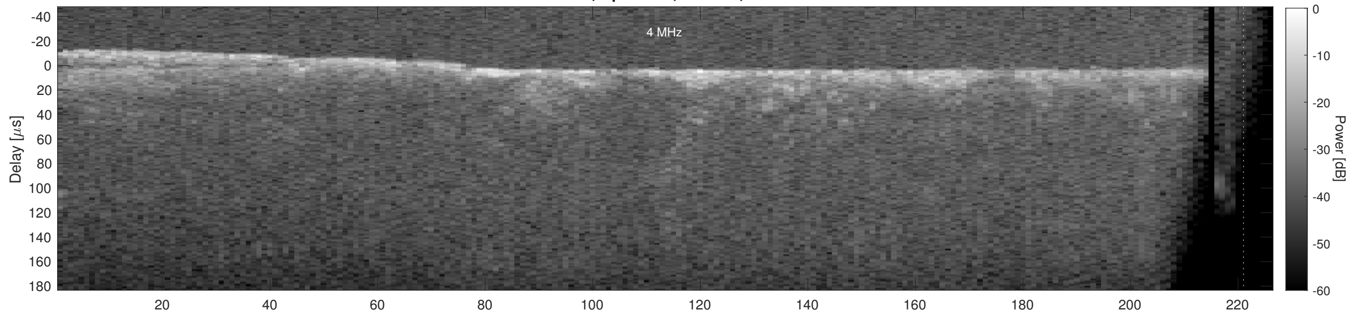
Orbit 18337, Cluttergram
