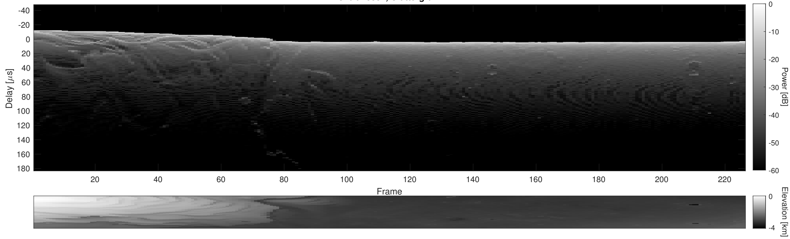
Orbit 18337, Cluttergram
