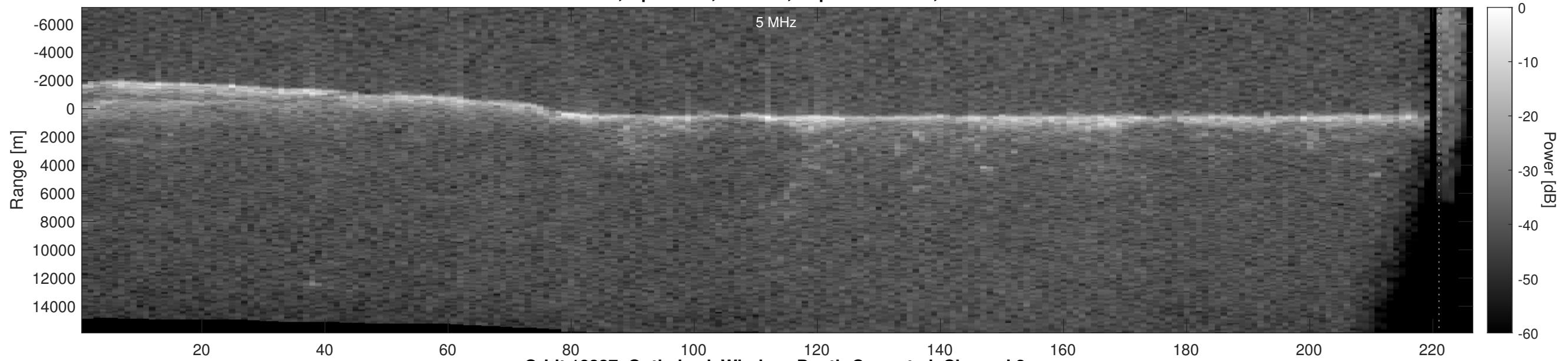
Orbit 18337, Optimized, Window, Depth-Corrected, Channel 2
