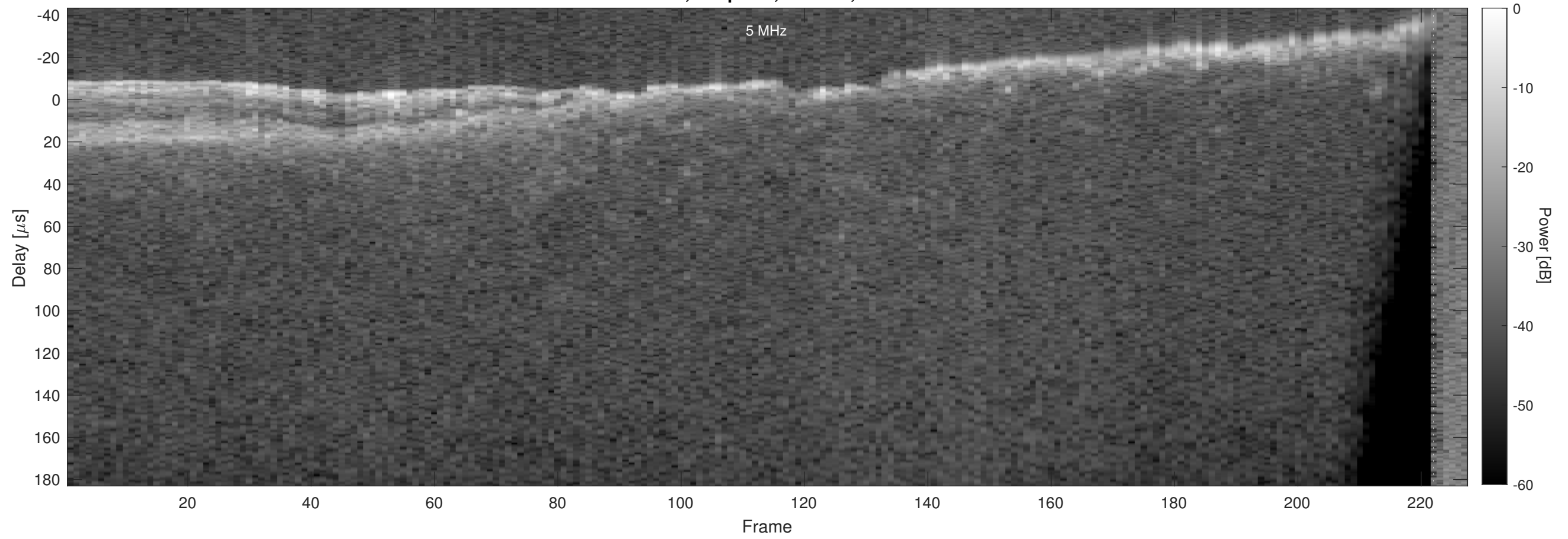
Orbit 18339, Chapman, Window, Channel 2
