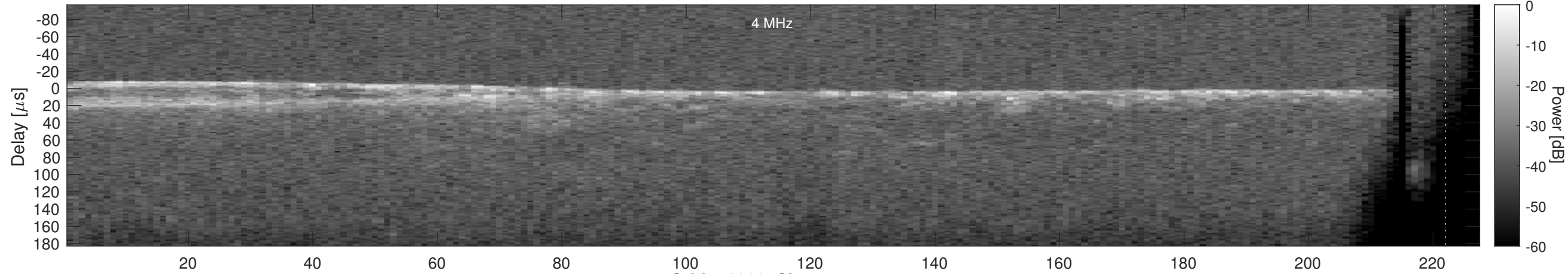
Orbit 18339, Cluttergram
