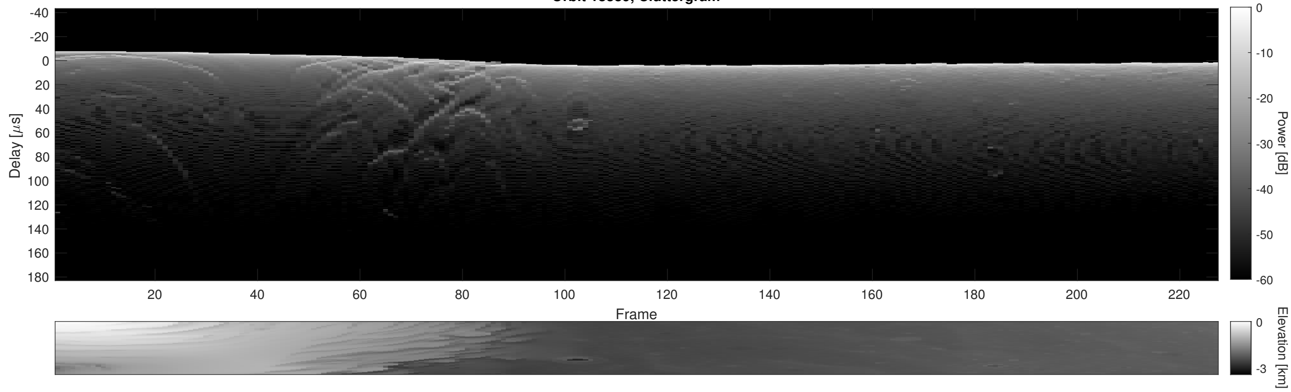
Orbit 18339, Cluttergram
