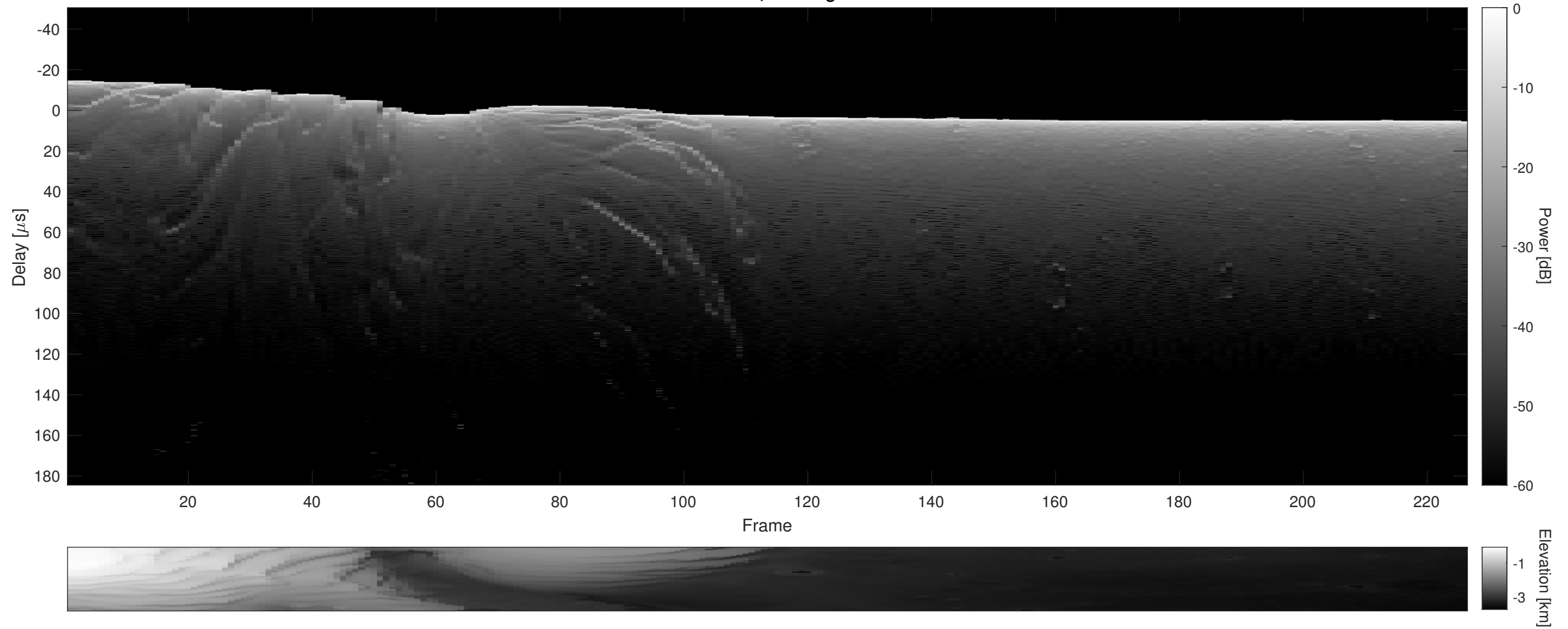
Orbit 18340, Cluttergram
