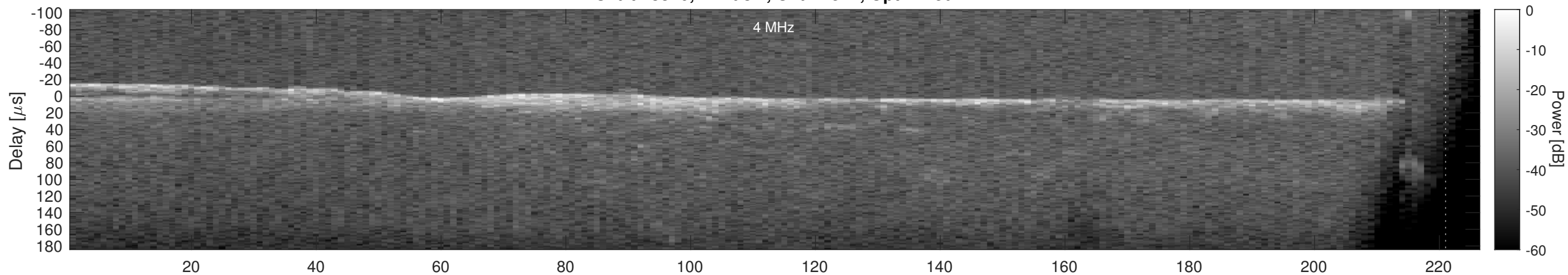
Orbit 18340, Cluttergram
