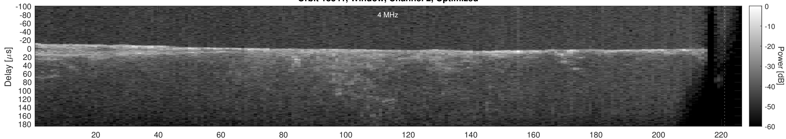
Orbit 18341, Cluttergram
