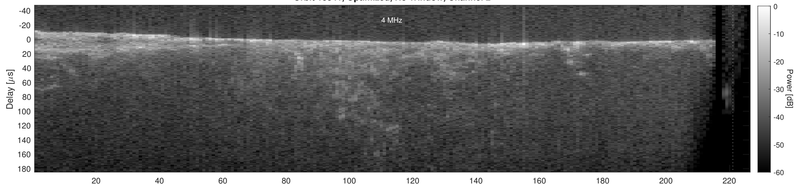
Orbit 18341, Cluttergram
