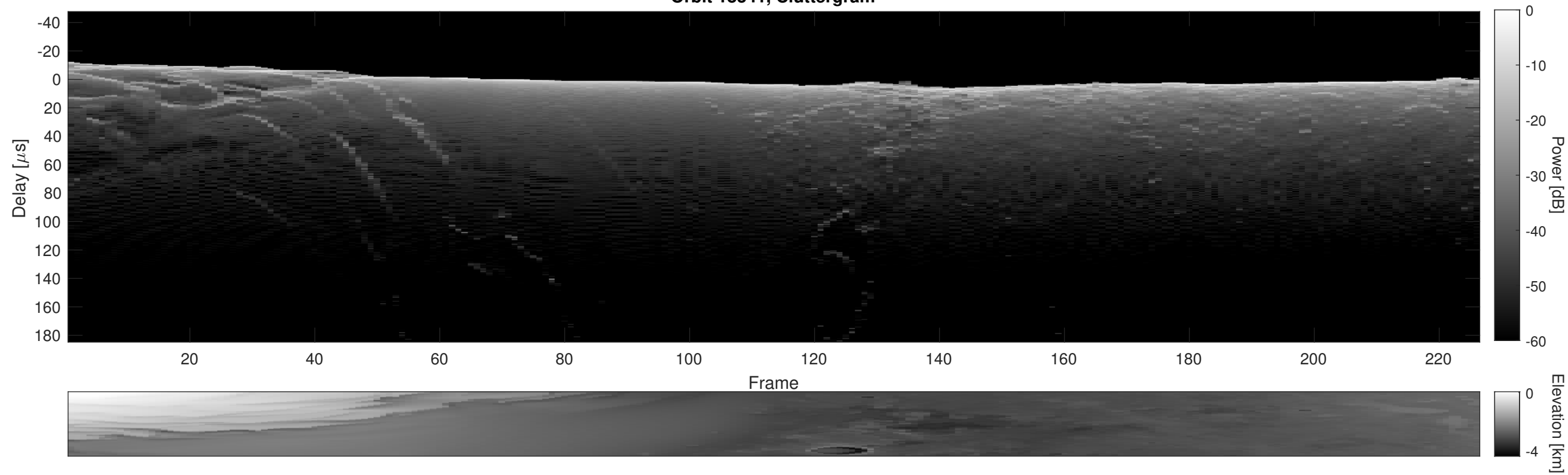
Orbit 18341, Cluttergram
