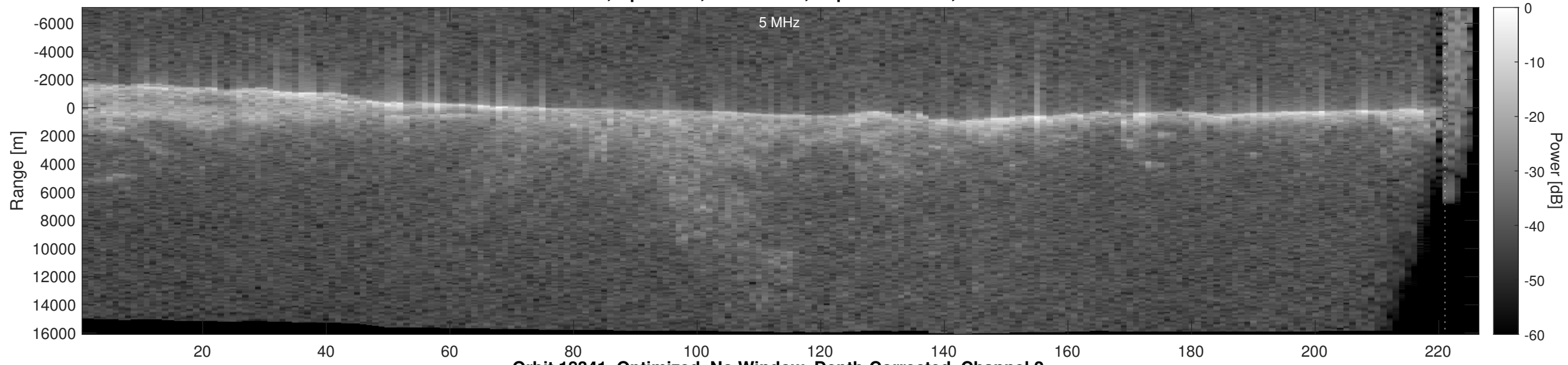
Orbit 18341, Optimized, No Window, Depth-Corrected, Channel 2
