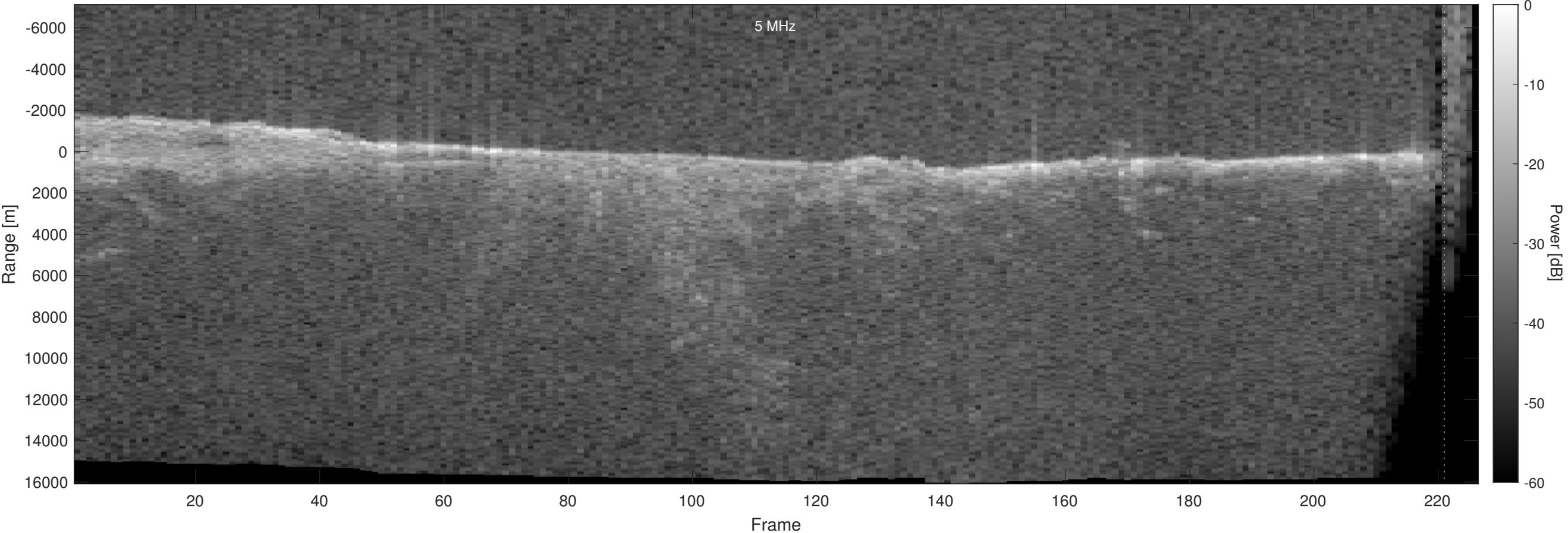
Orbit 18341, Optimized, Window, Depth-Corrected, Channel 2
