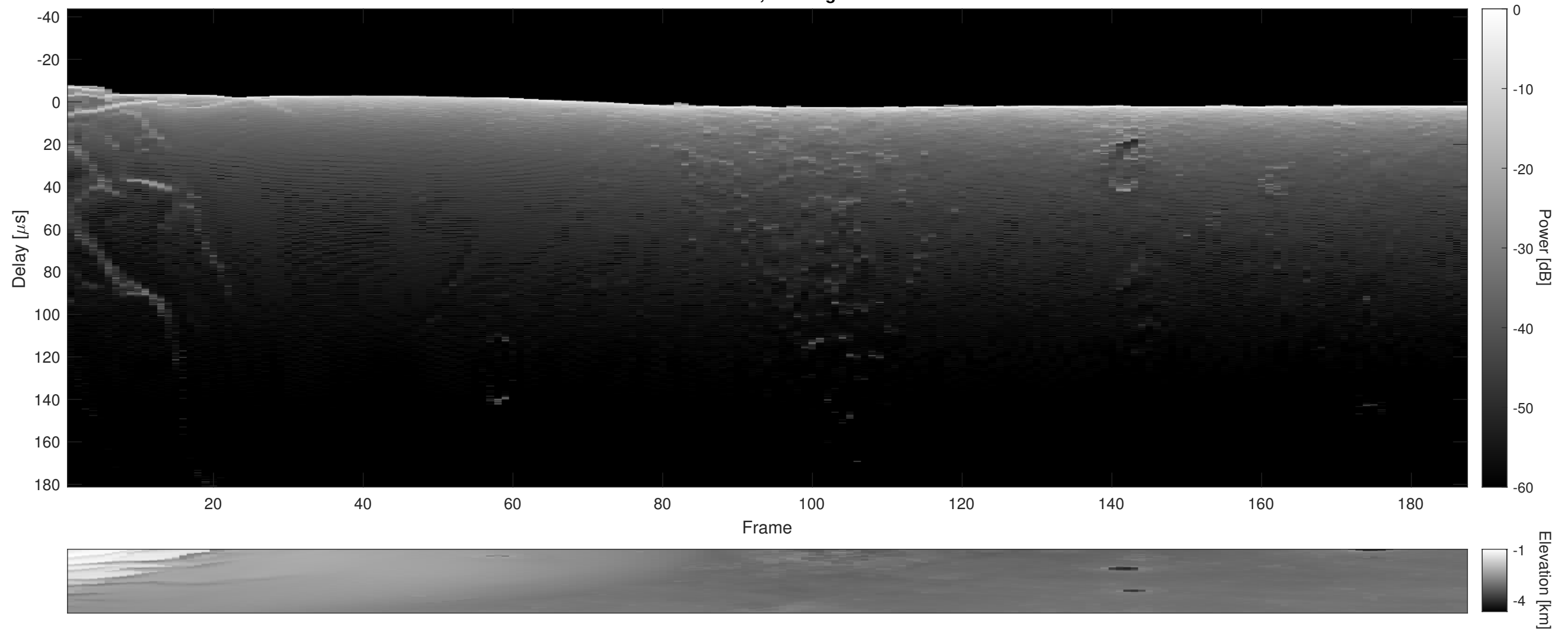
Orbit 18345, Cluttergram
