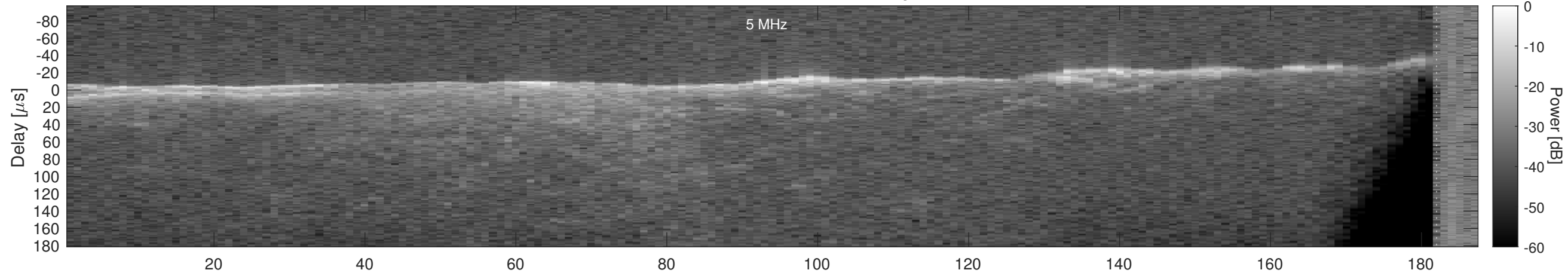
Orbit 18345, Window, Channel 1, Optimized
