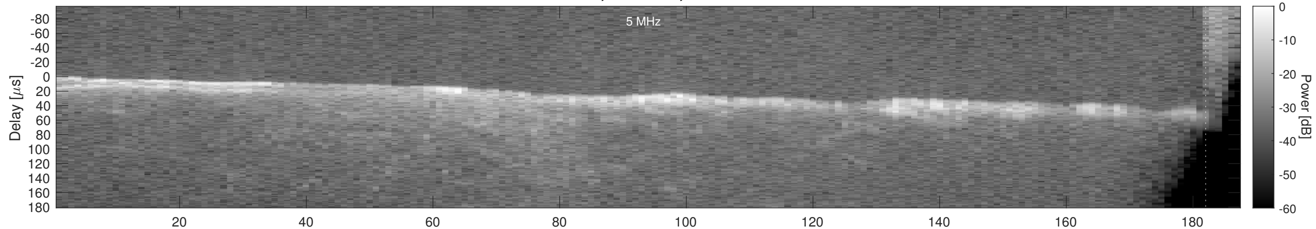
Orbit 18345, Window, Channel 1, Chapman
