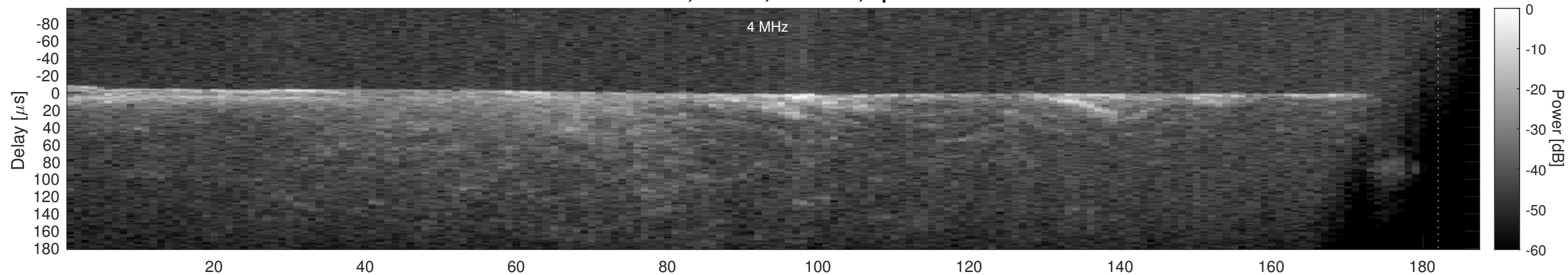
Orbit 18345, Cluttergram
