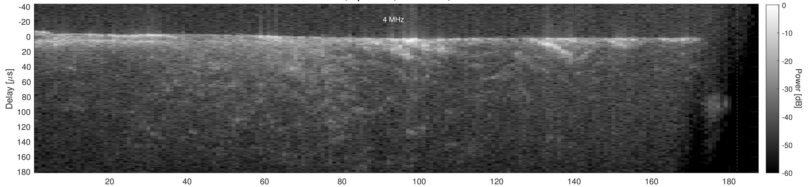
Orbit 18345, Cluttergram
