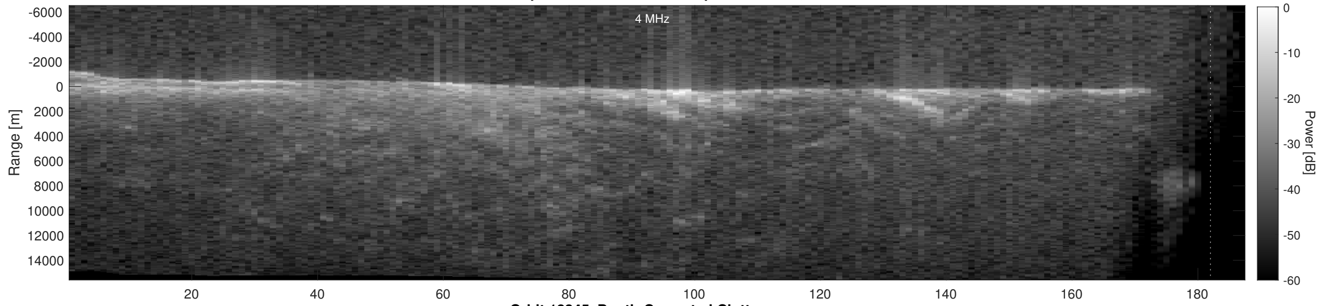
Orbit 18345, Depth-Corrected Cluttergram
