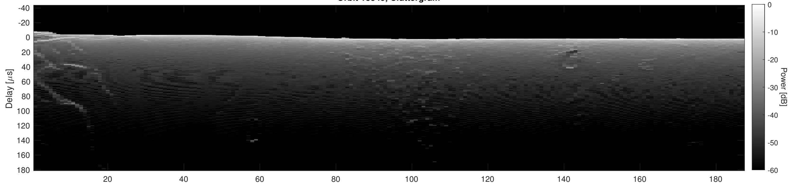
Orbit 18345, Cluttergram
