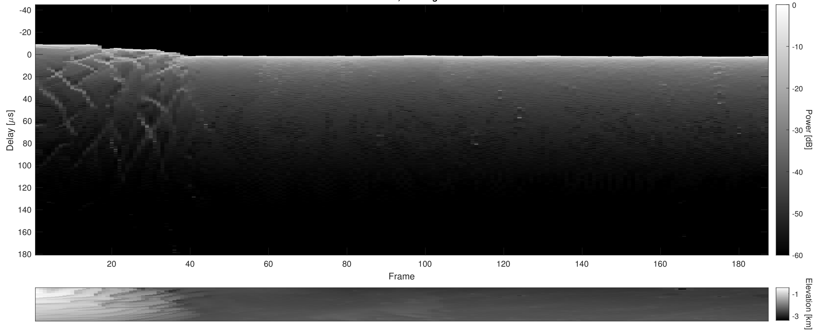
Orbit 18349, Cluttergram
