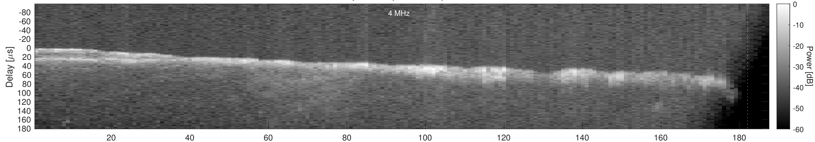
Orbit 18349, Window, Channel 2, Chapman
