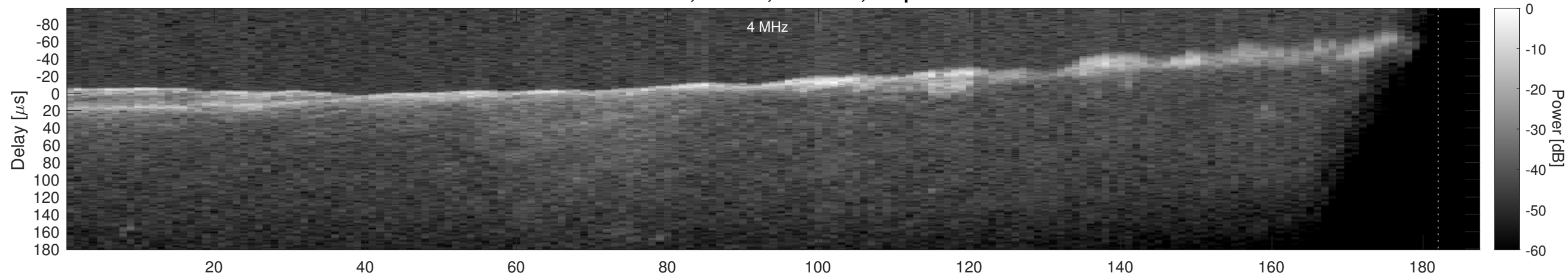
Orbit 18349, Window, Channel 2, Optimized
