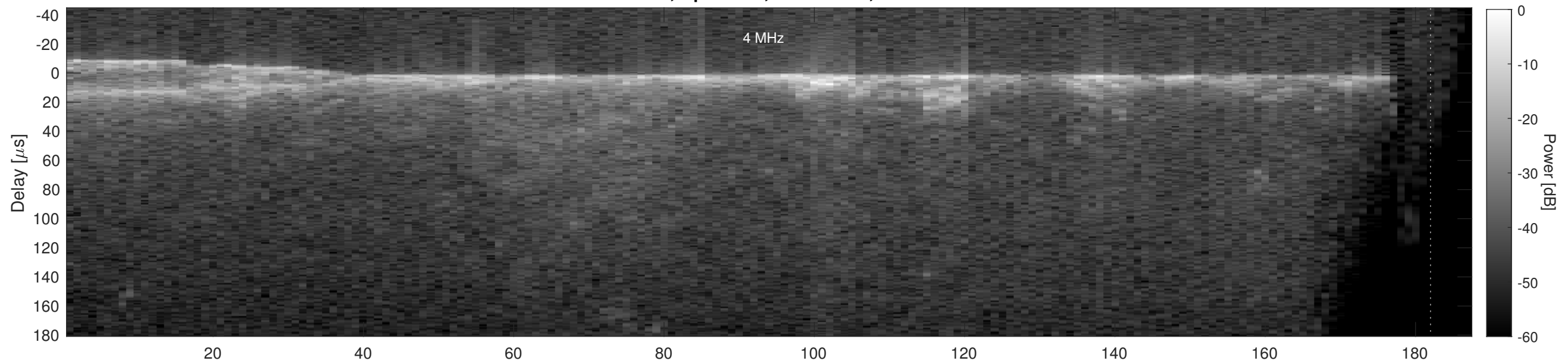
Orbit 18349, Cluttergram
