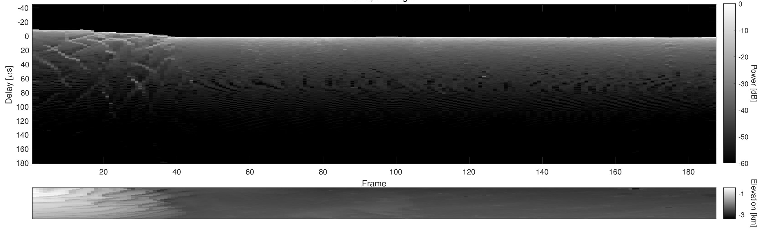
Orbit 18349, Cluttergram
