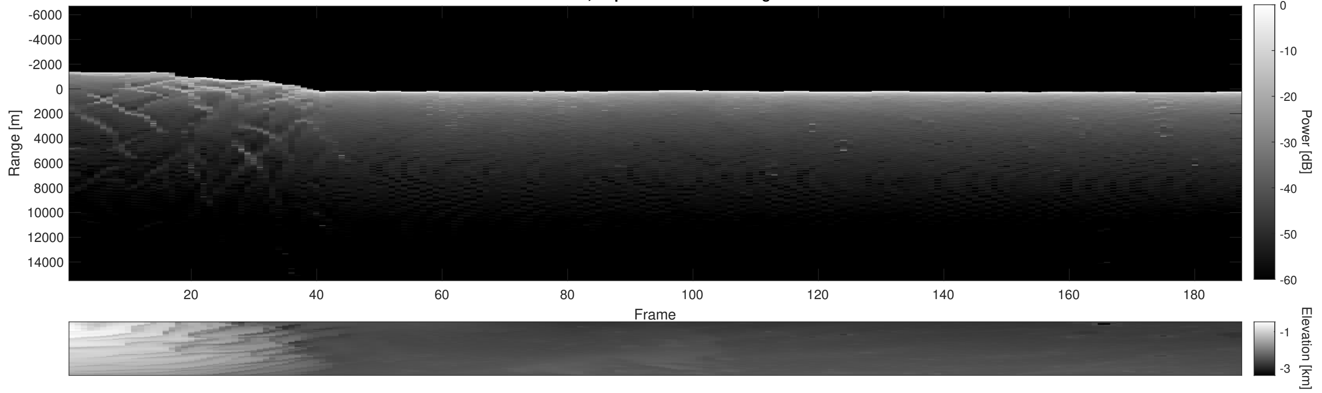
Orbit 18349, Depth-Corrected Cluttergram
