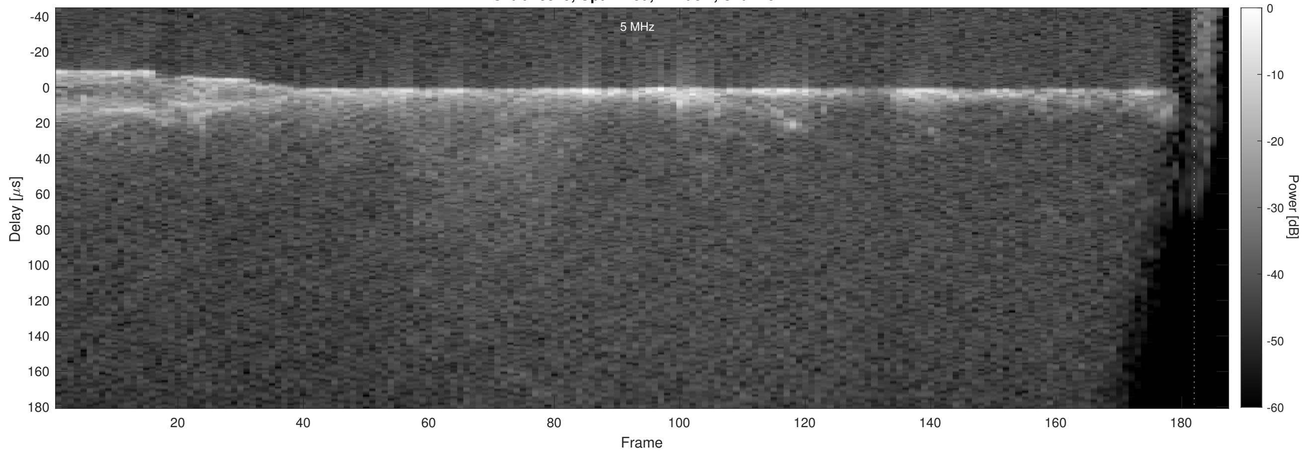
Orbit 18349, Optimized, Window, Channel 2
