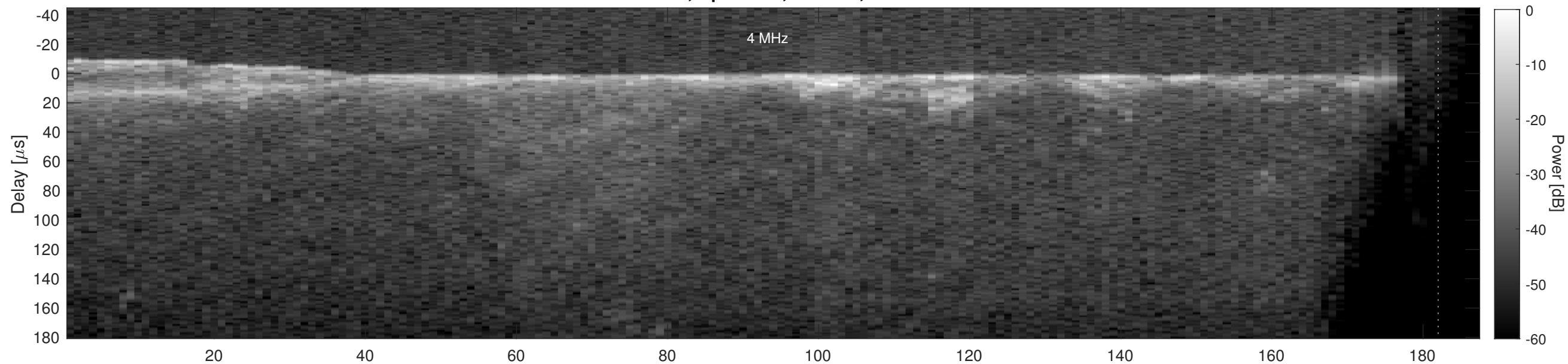
Orbit 18349, Cluttergram
