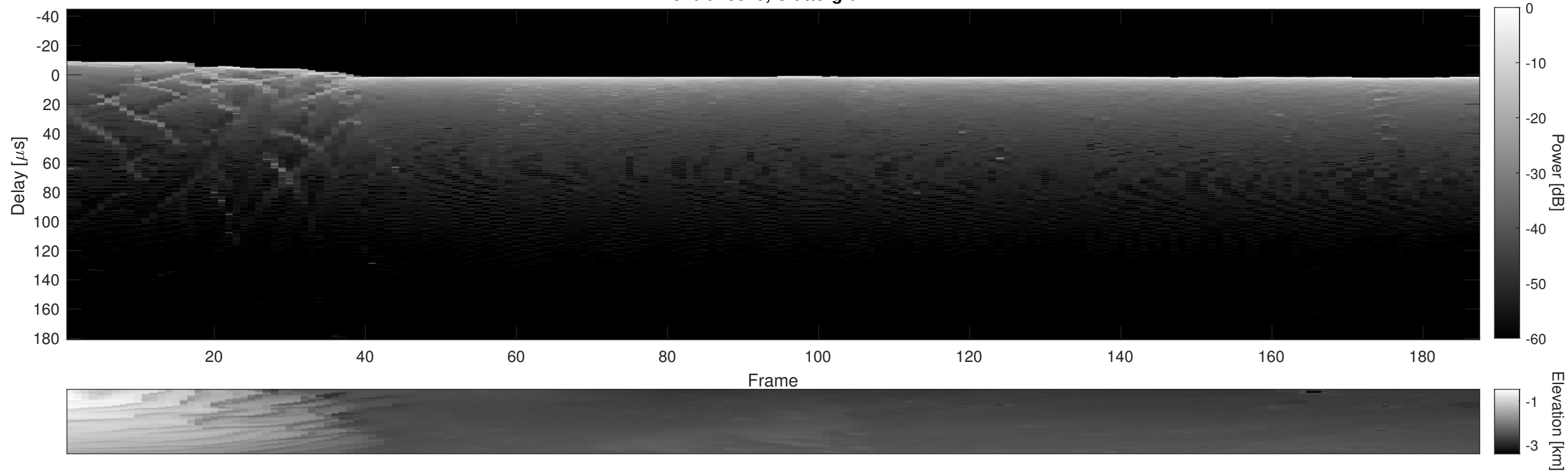
Orbit 18349, Cluttergram
