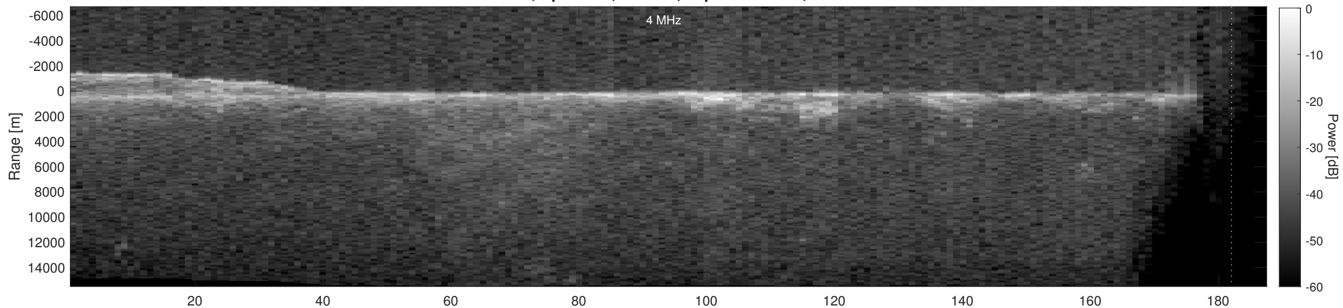
Orbit 18349, Depth-Corrected Cluttergram
