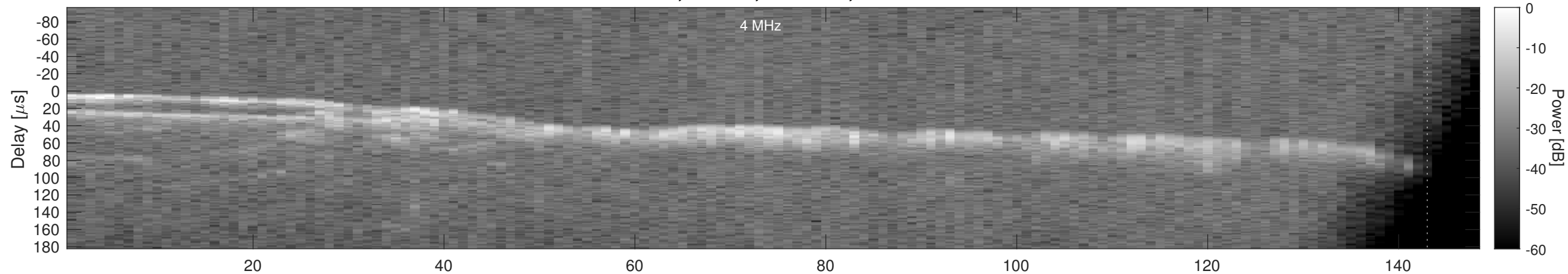
Orbit 18350, Window, Channel 2, Chapman
