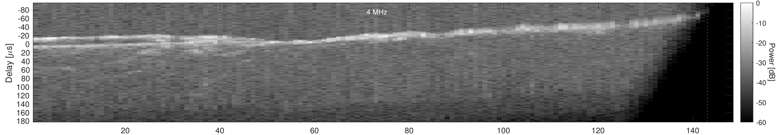
Orbit 18350, Window, Channel 2, Optimized
