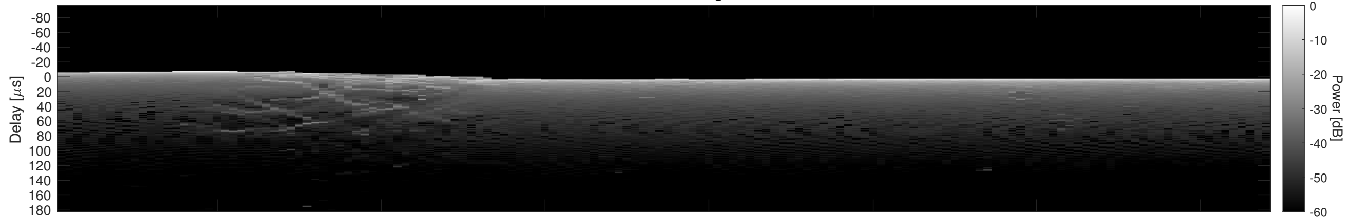
Orbit 18350, Cluttergram
