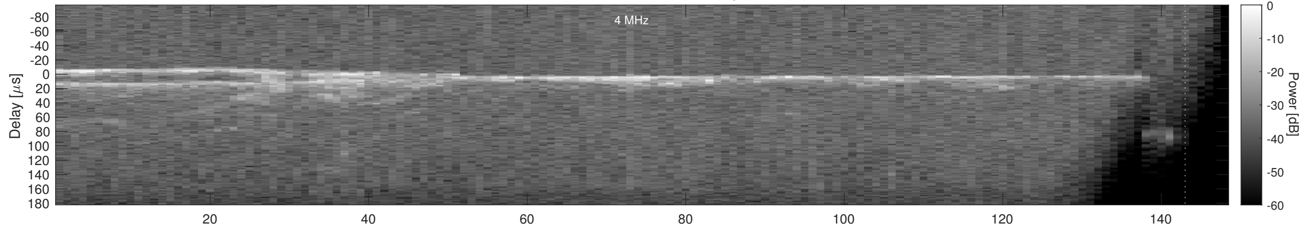
Orbit 18350, Cluttergram
