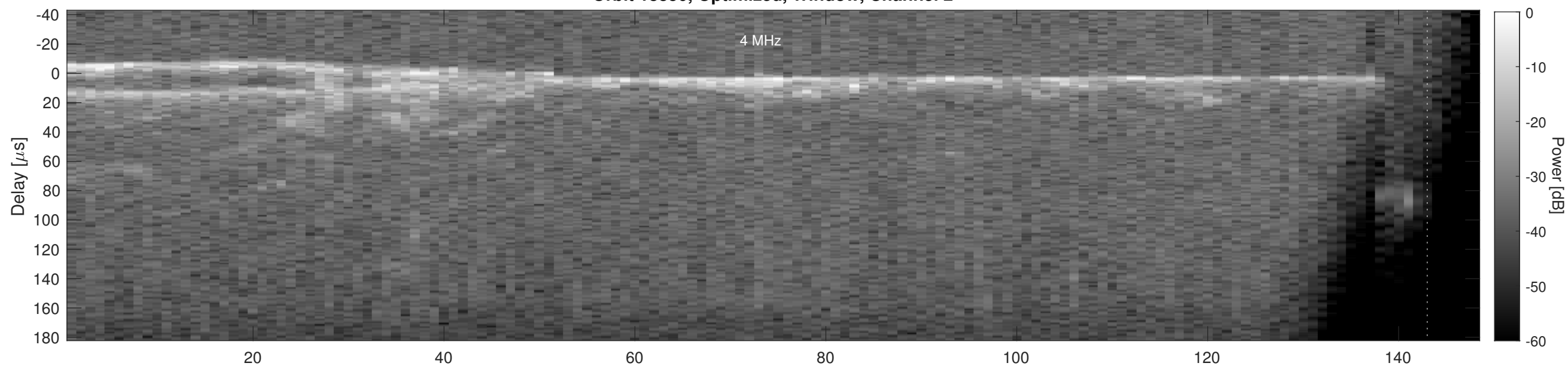
Orbit 18350, Cluttergram
