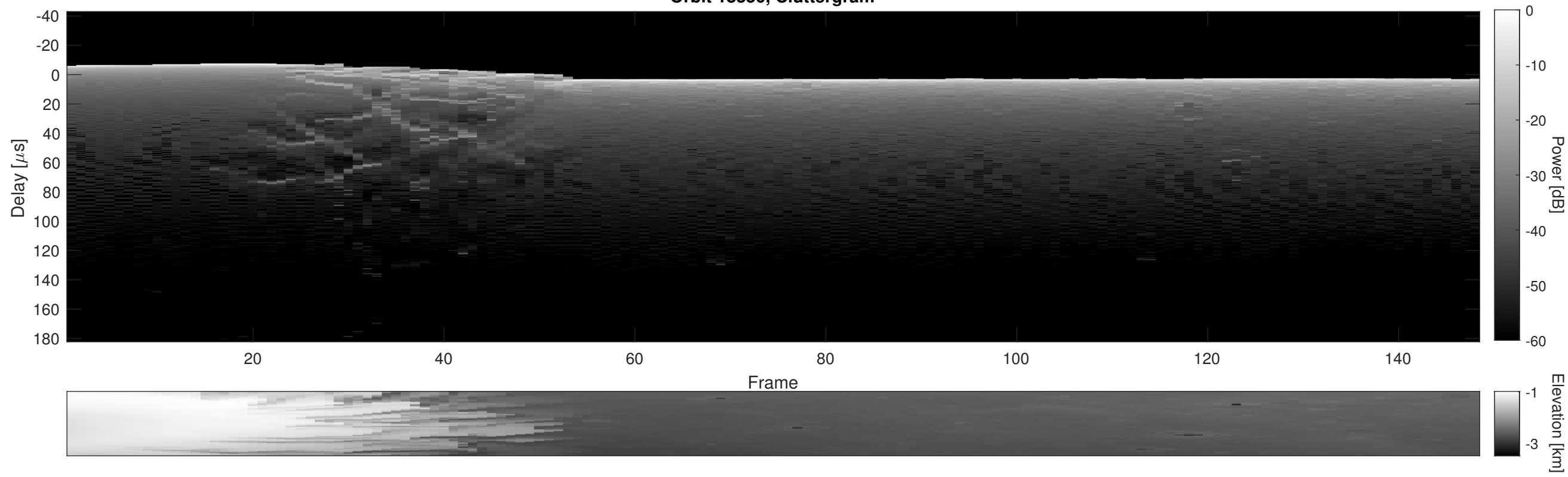
Orbit 18350, Cluttergram
