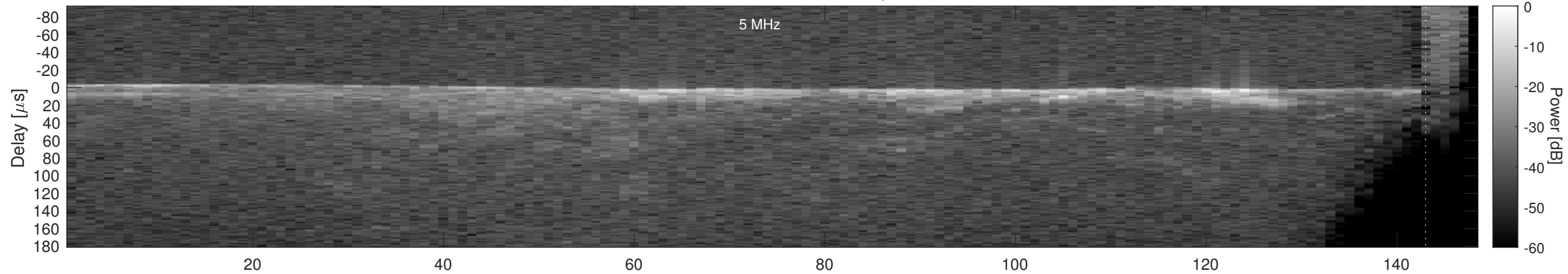
Orbit 18352, Cluttergram
