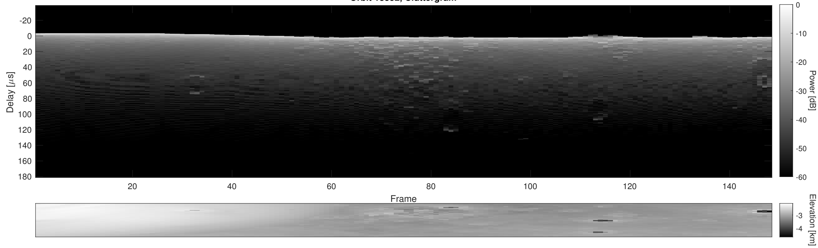
Orbit 18352, Cluttergram
