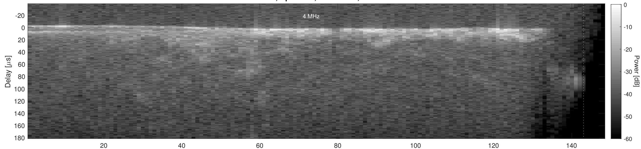
Orbit 18352, Cluttergram
