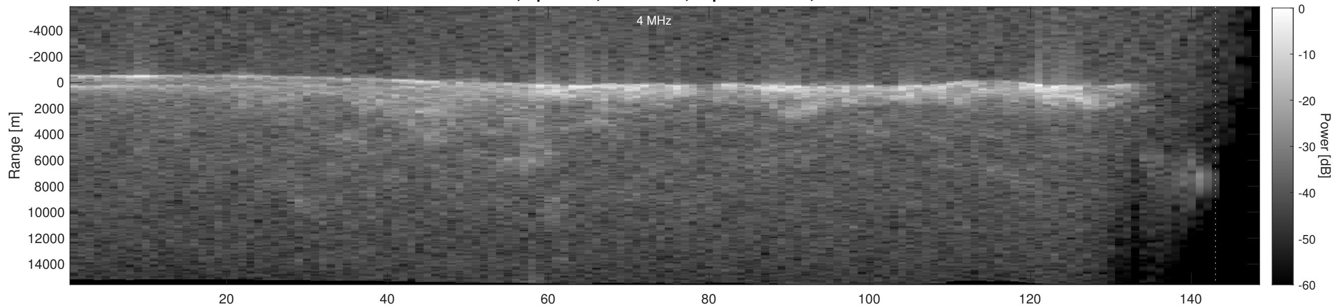
Orbit 18352, Depth-Corrected Cluttergram
